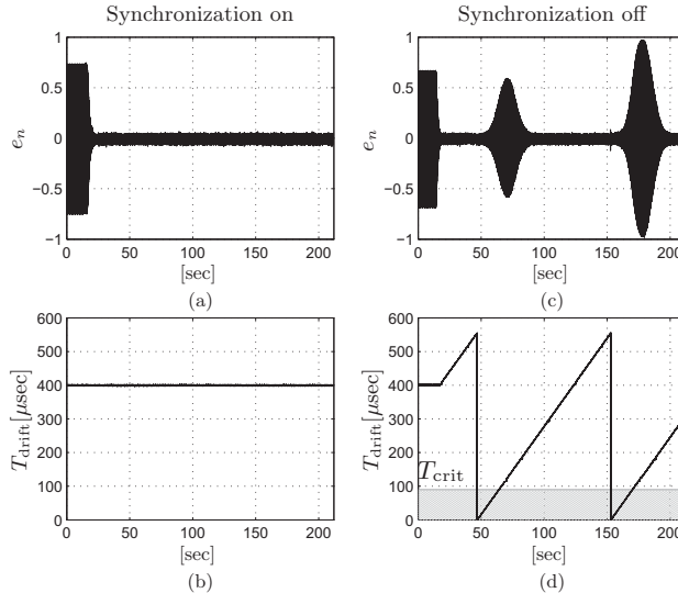
Fig. 5. Measurement results in an ANC system. (a) and (c): noise signal measured by the external microphone when synchronization is on and off, respectively. (b) and (d): delay ( T_{\text{drift}} ) between the notes when synchronization is on and off, respectively.
