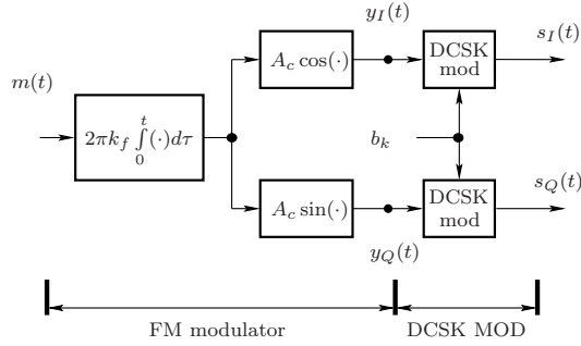
Fig. 2. BB equivalent of FM-DCSK modulator.
