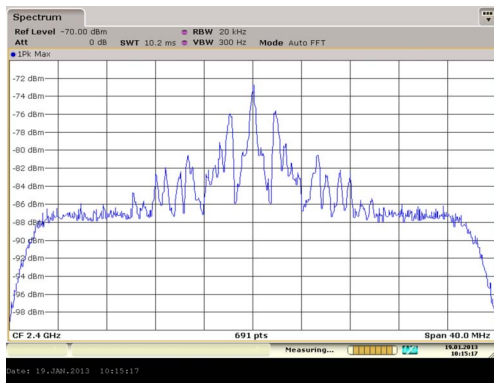
Fig. 8. Measured spectrum of FM-DCSK in office environment.
