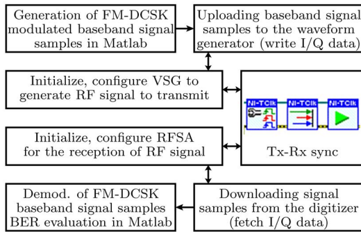
Fig. 6. Block diagram of the SW components of the wireless platform
