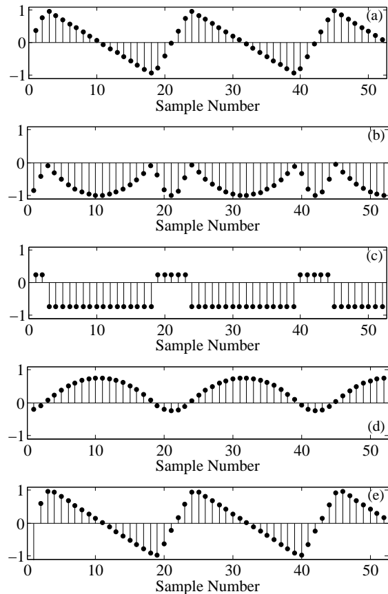
Figure 2. Generation of the triangle signal with variable symmetry. (a) The trivial signal is first processed with the x^2 - 1 function. (b) The result is then multiplied with (c) a scaled rectangular wave to get (d) the parabolic waveform. Finally differentiating and scaling produce (e) the desired alias-suppressed waveform.
