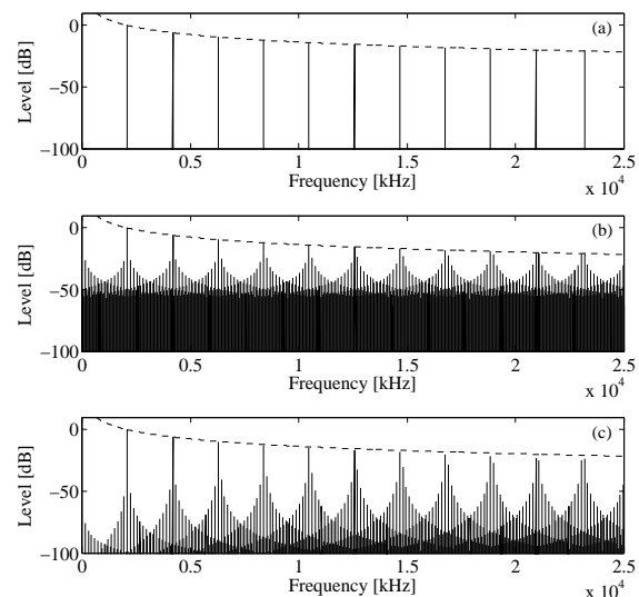
Figure 1. Spectrum of (a) the ideal, (b) the trivial and (c) the DPW sawtooth signals. The dashed line is the envelope of the ideal spectrum.
